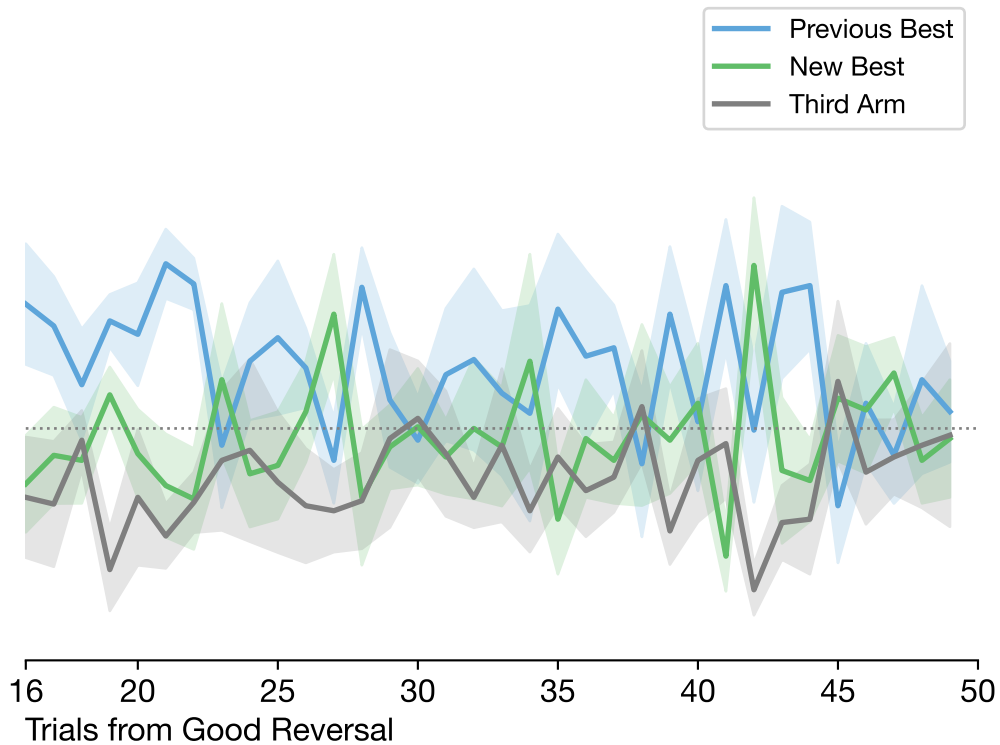
Good Reversal-Aligned Choices (mean \pm se across subjects | n=6 subjects, n=26 reversals) (Skipping first 15 trials post-reversal)
